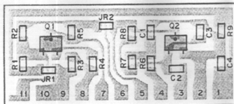
AF PRE AMP (X59-1110-00) Component side view
