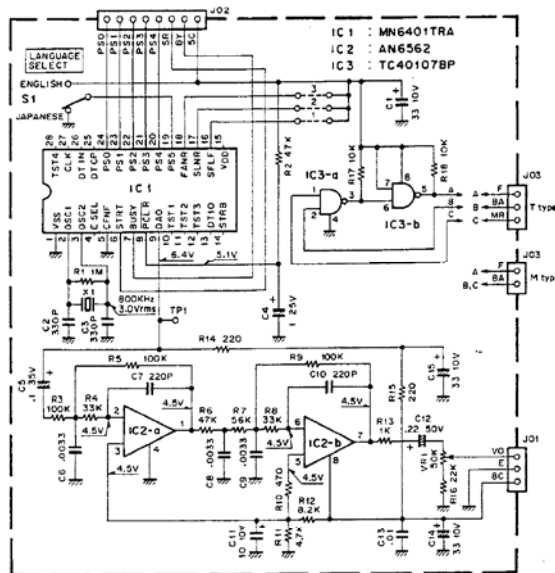
VS-1 SCHEMATIC DIAGRAM
