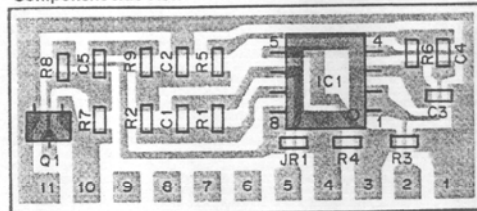
MIC AMP (X59-3000-01) Component side view
